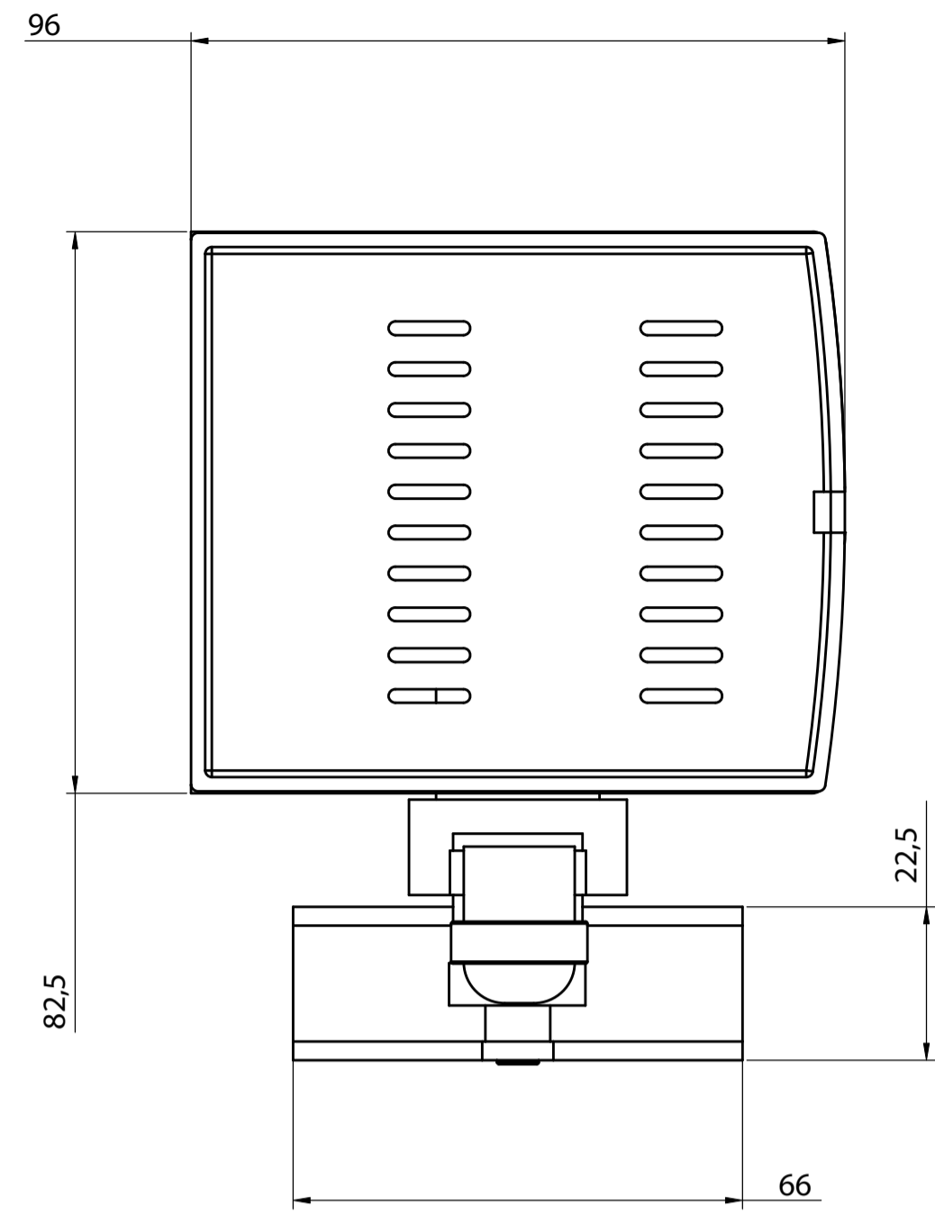
Side view
